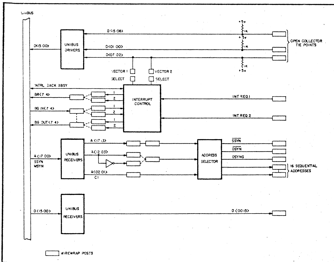
Figure 1 MDB-1710, Block Diagram
